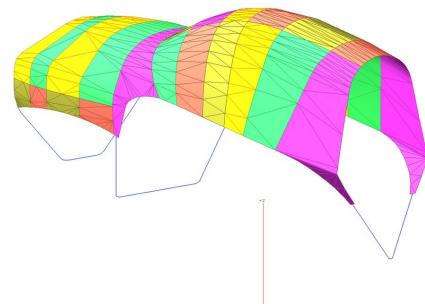
SAW Revo Canopy Cover w/fwd extension, 3D model
