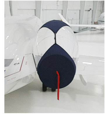
Intake/Exhaust Covers, 3-Strap Type. Successfully installed by two crew, one Challenger 300 Intake/Exhaust Cover Set, 3-strap ladder. type
