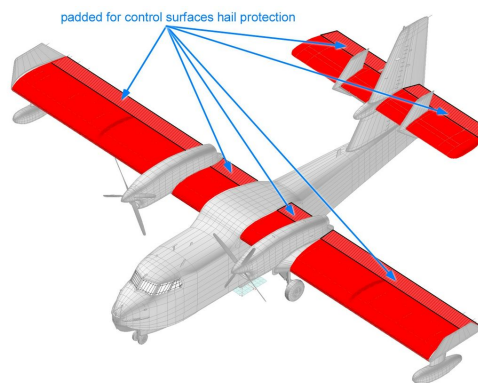
Canadair CL-415 Super Scooper Hail Protection Control Surfaces Covers
