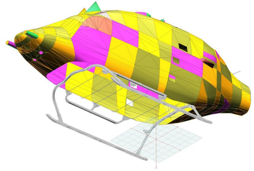
Bell 429 Main Body Cover, 3D model
